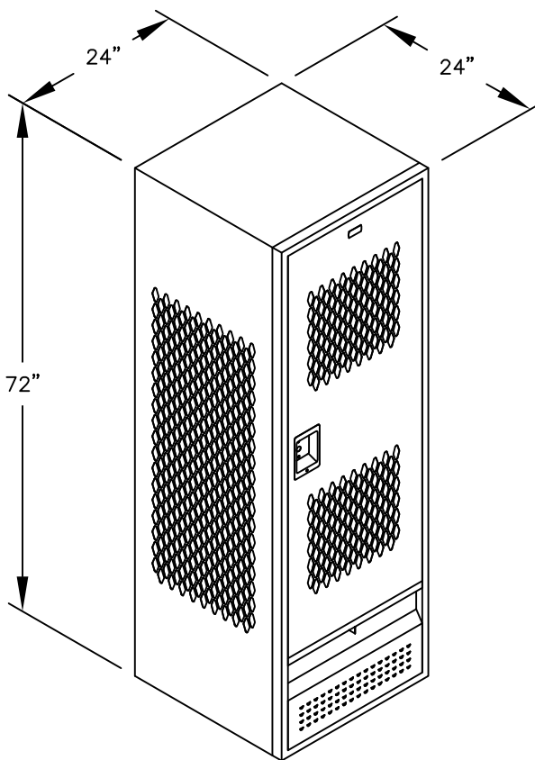
MODEL #72024 24" WIDE STANDARD GEAR LOCKER WITH VENTILATED DOOR
